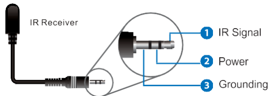
IR RECEIVER
